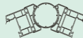
multi-angle corner adaptor
