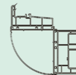
88 bay corner adaptor
