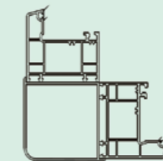
60 bay corner adaptor
