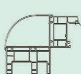
80-60 corner adaptor
