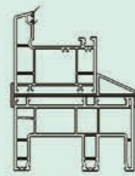
88-60 flat board
